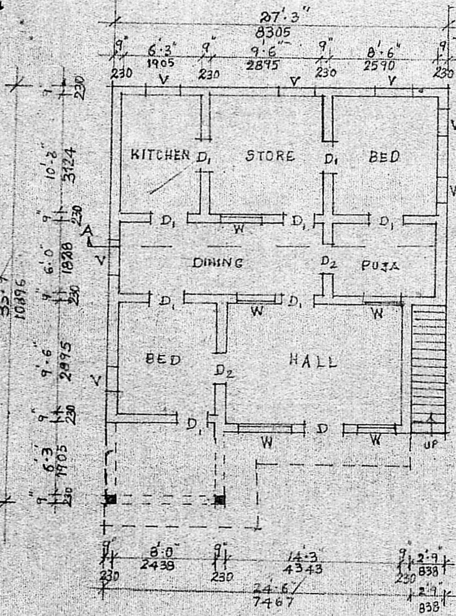
G.F. PLAN
